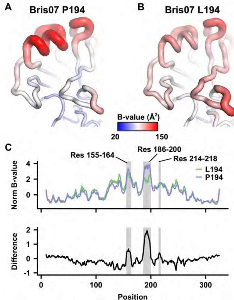
Fig 2. B-value analysis of Bris07 HA. (A–B) B-values (Å 2 ) of Ca atoms in (A) Bris07 P194 and (B) Bris07 L194 are projected on the HA structure. Of note, on average, the B-values of Ca atoms in Bris07 P194 (mean ± s.d. = 58 ± 24 Å 2 ) are lower than that of Bris07 L194 (mean ± s.d. = 64 ± 24 Å 2 ). (C) The normalized B-values of Ca atoms in Bris07 P194 (blue) and L194 (green) are compared. The bottom panel shows their difference in HA1: (normalized B-values of Ca atoms in P194) ± (normalized B-values of Ca atoms in L194). The amino-acid position is plotted along the x-axis. Positions corresponding to the residues (Res) of interest are shaded in grey.
