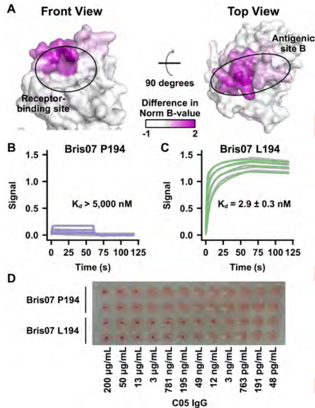
Fig 3. Impact of L194P substitution on antigenicity. (A) The difference in normalized B -values between Bris07 P194 and Bris07 L194 ( B -value Diff.) for each C \alpha atom is projected on the HA structure of Bris07 L194. B -value Diff. = (normalized B -values of C \alpha atoms in P194) \pm (normalized B -values of C \alpha atoms in L194). (B-C) Biolayer interferometry (BLI) was used to measure the binding kinetics of C05 IgG against the recombinant HA proteins of (B) Bris07 P194 and (C) Bris07 L194. (D) HAI assay of C05 IgG against Bris07 P194 and Bris07 L194 viruses. Duplicates were performed for each of Bris07 P194 and L194.
